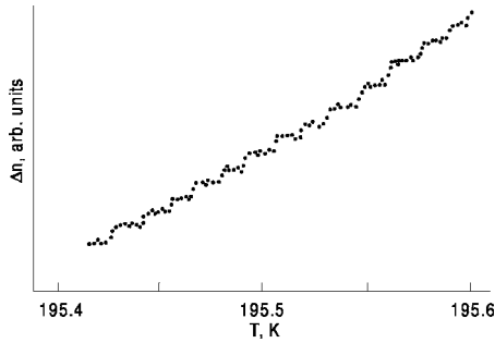
Fig. 2. Temperature dependence of birefringence of \text{Sn}_2\text{P}_2\text{Se}_6 incommensurate phase at the temperature change rate 0.4 K/hours [6].
