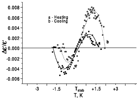
Fig. 9. Temperature dependence of the reduced anomalous part of the dielectric constant associated with the memory effect (from Figure 6) at heating and cooling regimes.
