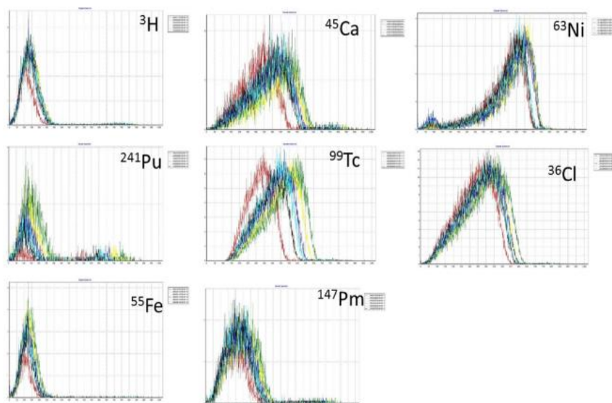
Fig. 2 Examples of spectral shift of beta spectra due to the presence of quench in analysed samples. SQPE range: ^3\text{H} (642–722), ^{241}\text{Pu} (473–756), ^{55}\text{Fe} (673–777), ^{45}\text{Ca} (624–746), ^{99}\text{Tc} (570–750), ^{147}\text{Pm} (674–760), ^{63}\text{Ni} (661–756), ^{36}\text{Cl} (631–683)
