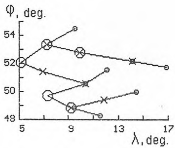
Figure 6. Geographical coordinates reference A (O) and researched B, C (x, o) points
