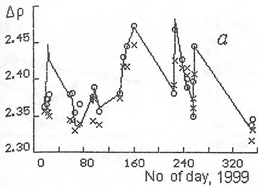
Figure 3. Change of the correction \Delta\rho (meters) by results of night explorations of atmosphere in Uzhhorod in 1999 (line); o – the same corrections with the eliminated inversions of temperature (a) or damp (b); x – corrections calculated by the Saastamoinen formula
