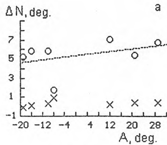
Figure 7. Differences \Delta N of refraction indexes of spherically symmetrical model and meteorological atmosphere for different azimuths A (zenith distance z = 88^\circ ) at the altitude 6 km in points B (o) and 26 km in C (x) at night (a) and in the day-time (b)
