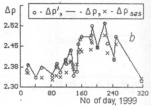
Figure 3. Change of the correction \Delta\rho (meters) by results of night explorations of atmosphere in Uzhhorod in 1999 (line); o – the same corrections with the eliminated inversions of temperature (a) or damp (b); x – corrections calculated by the Saastamoinen formula
