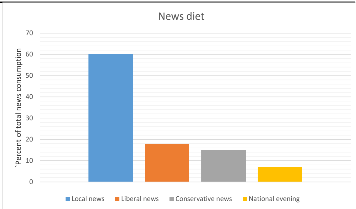
Graph 1. News diet, cited in [21, p.117]
