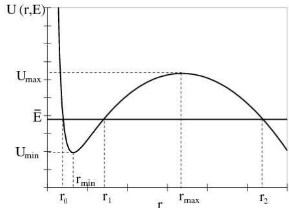
Fig. 1. Form of the barrier-type effective potential U(r, E) ; \bar{E} = (E^2 - m^2)/2m is the effective energy; r_0, r_1 and r_2 are roots of equation p^2(r) = 0 .
