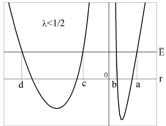
Fig. 2. The effective potential U(r, E) with potentials (4), (5) in the case 0 \leq \lambda < 1/2 , \sigma > 0 ; a, b, c and d are roots of quasimomentum p^2(r) = 0 .
