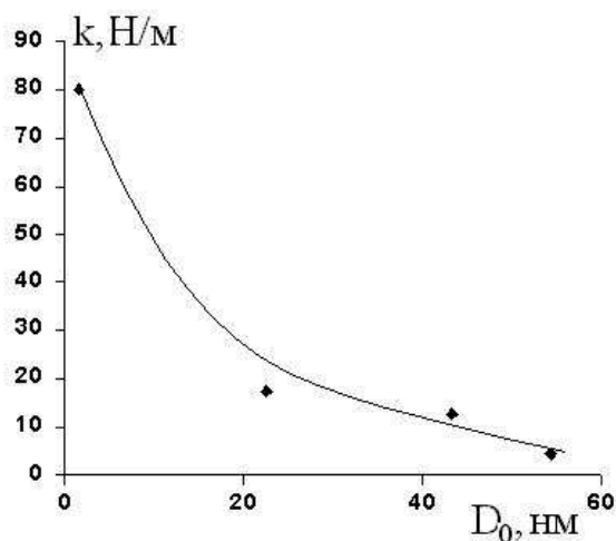
Fig. 3. The dependence of elastic coefficient of nanotubes over their diameter
