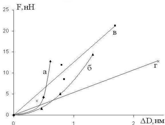
Fig. 2. The dependence of the force influence of probe over the nanotube from absolute deformation of the one for the single-walled nanotubes (a), multiwalled ones with diameter 43 nm (b), 22 nm (B) and 54 nm (r)
