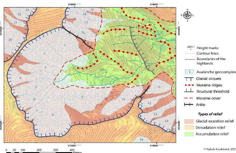
Figure 2 Avalanche geocomplexes on the walls of glacial cirques in the upper basin of the Mreye Stream (leeward north-eastern sector of Chornohora Landscape)
