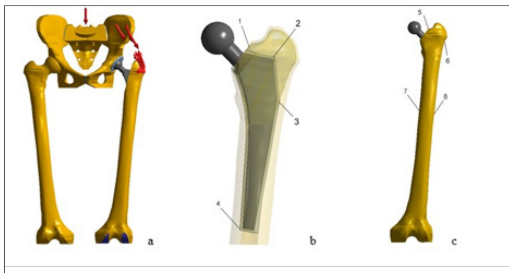
Fig. 2. Calculation model: a) Direction of action of forces and fixation of the model; b) control points in the frontal section of the femur; c) control points on the surface of the femur.
