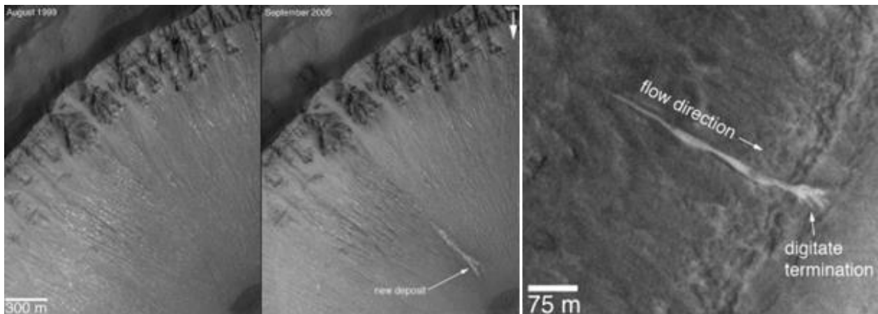
Fig. 1. On the left - an alluvial flow on the slopes of the crater in the Terra Sirenum area, which took place between 08.1999 and 09.2005. On the right - a possible light-colored mudflow in 2005 ( http://photojournal.jpl.nasa.gov/ ).
