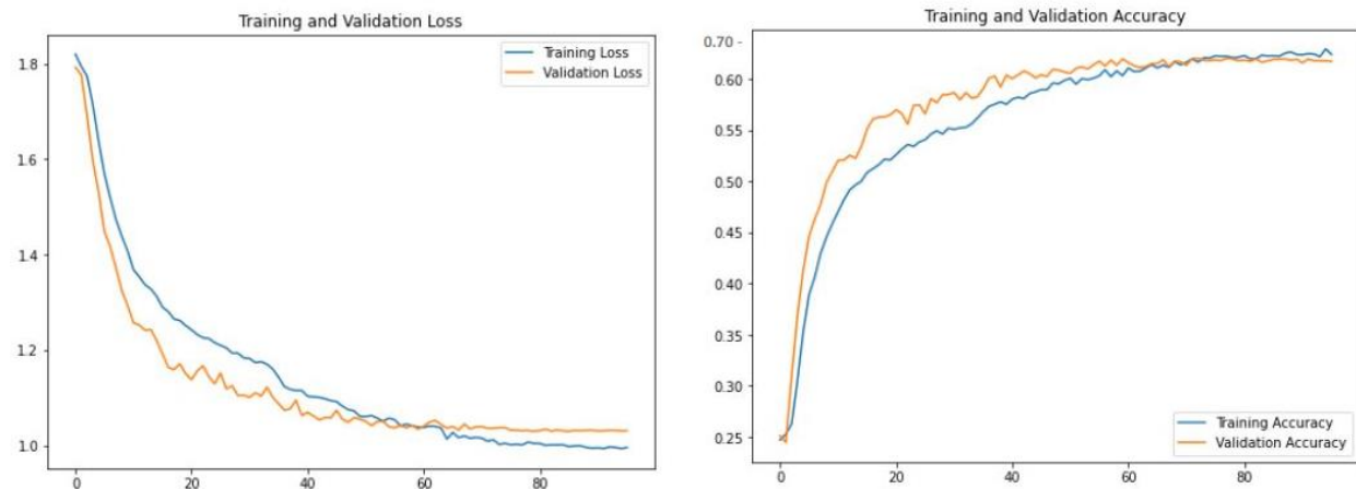
Fig. 6. Validation loss and Accuracy during training
