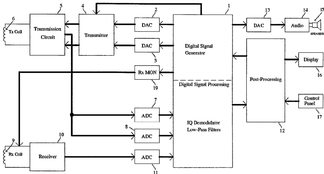
Figure 1 – Block diagram of Minelab equinox series metal detectors [7]
