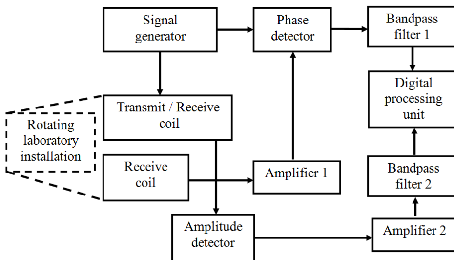
Figure 3 – The structural diagram of the modernized RS
