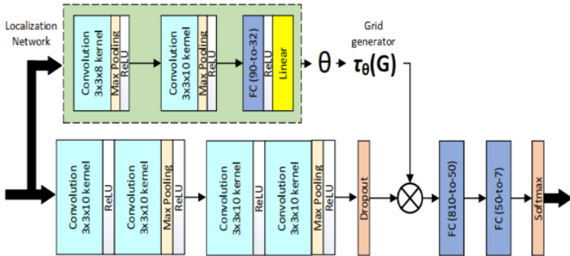
Fig. 4. Proposed architecture
