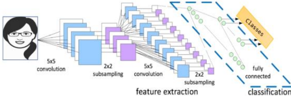
Fig. 2. CNN-based architecture for facial expression recognition [1]
