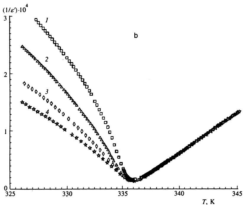
FIG. 1. The temperature curves of (a) \epsilon' and (b) 1/\epsilon' at different temperature variation rates: curves 1, 0.02 \text{ K min}^{-1} ; curves 2, 0.05 \text{ K min}^{-1} ; and curves 3, 0.2 \text{ K min}^{-1} .
