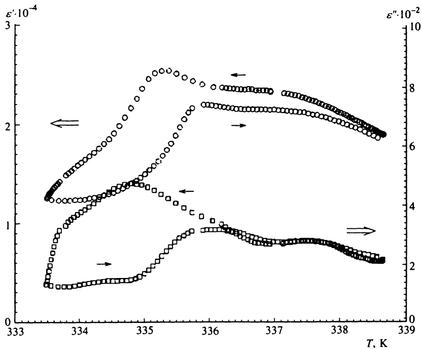
FIG. 3. The temperature hysteresis of \epsilon'(T) and \epsilon''(T) after exposing the sample to a temperature of T=336.2 K for six hours.
