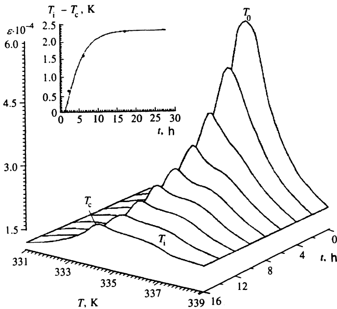
FIG. 2. The temperature curves of the dielectric constant of \text{Sn}_2\text{P}_2\text{S}_6 crystals after exposure at T=336.2 K. The inset depicts the temporal dependence of the temperature interval T_i - T_c at the same exposure temperature (the \circ symbols stand for the experimental data, and the curve represents the theoretical results).
