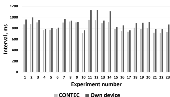
Fig. 7. Results of measurement of R-R intervals (light color) and peak-peak intervals (dark color) with two devices
