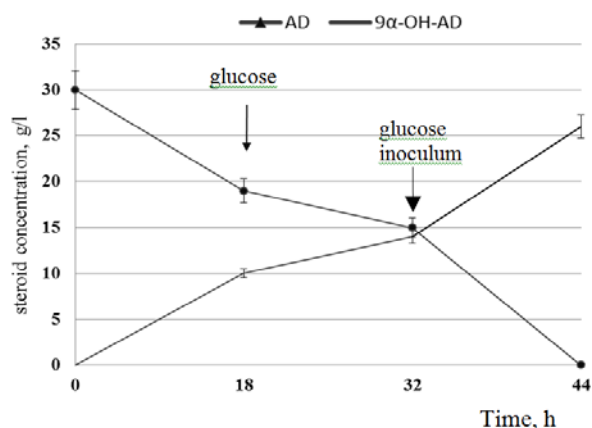
Fig. 3. Dynamics of 9α-OH-AD accumulation at the AD load of 30 g/l
