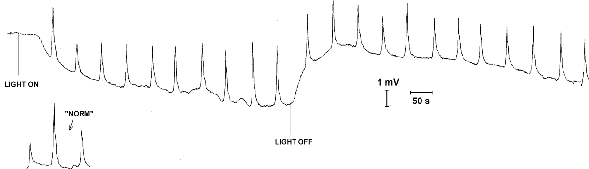
Fig. 8. Dynamics of the amplitude of "cold" potentials caused by rhythmic cold irritations \Delta t = -5^\circ\text{C} duration 5 seconds against the background of photopotential with continuous light stimulation with white light with illumination of 250 lux
