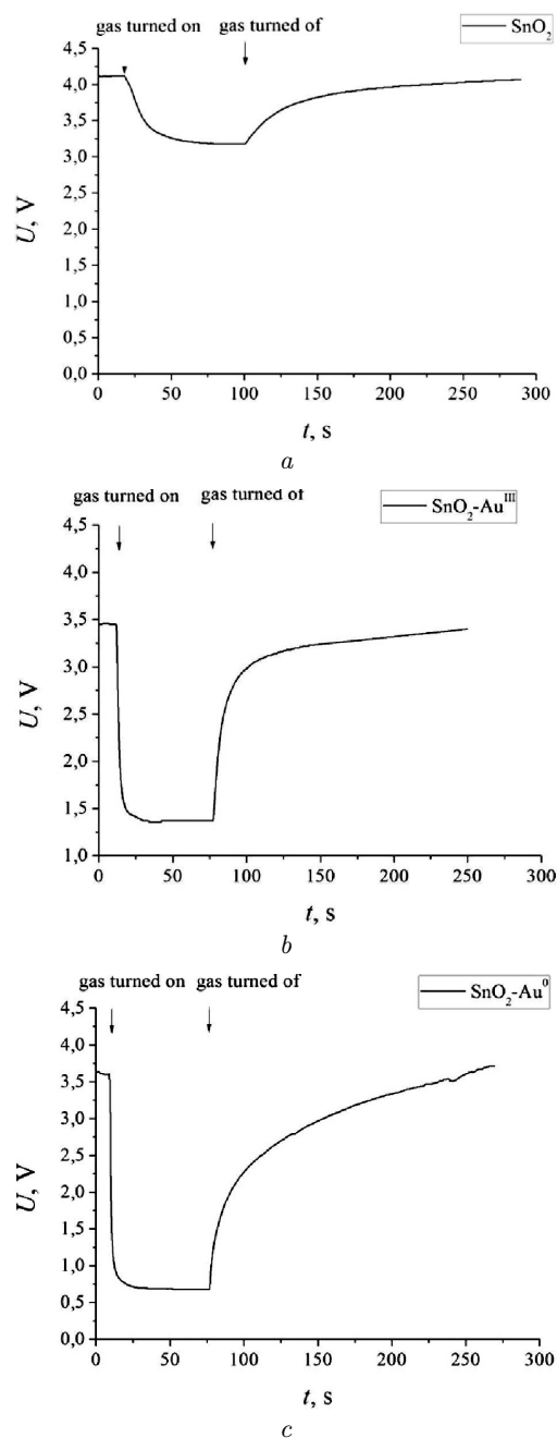
Fig. 3. Dynamic characteristics of the SnO 2 (a), SnO 2 -Au III (b), and SnO 2 -Au 0 (c) sensors under detection of acetone vapors (10 ppm)
