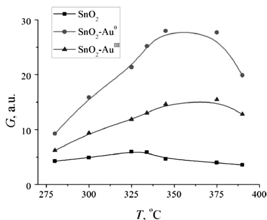
Fig. 2. The sensor response vs working temperature graphs of the SnO 2 , SnO 2 -Au III , and SnO 2 -Au 0 sensors under detection of acetone vapors (50 ppm)
