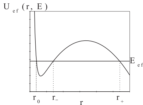
Figure 1. The type of the effective potential U_{ef}(r, E) .
